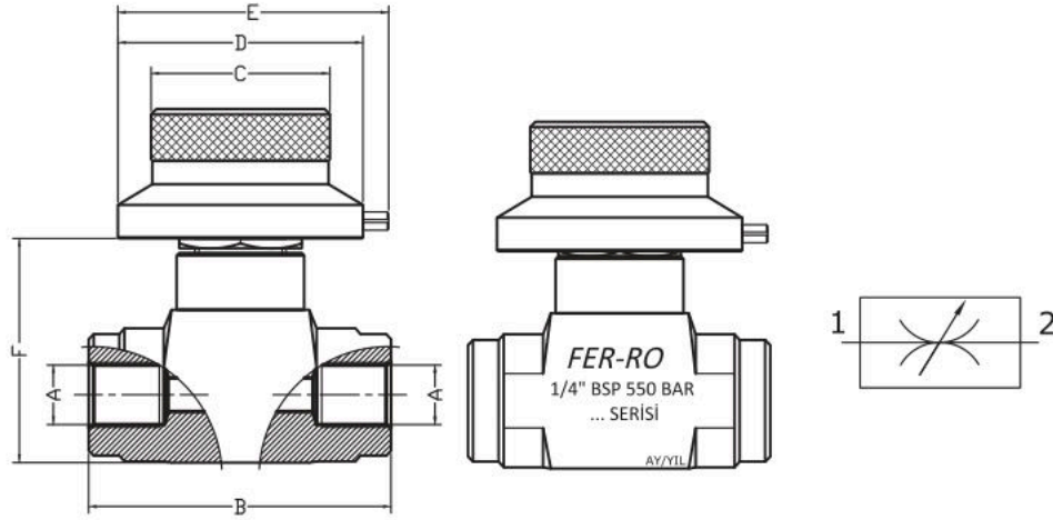
YANDAN GİRİŞ / INLINE CONNECTION
