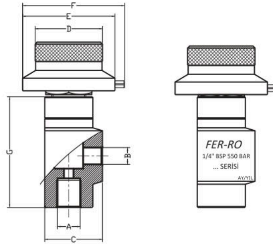
ALTAN GİRİŞ / REAR CONNECTION
