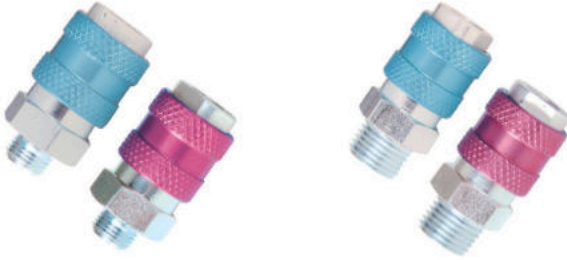
PN21G18MCN - 1/8" BSP Erkek Gövde / 1/8" BSP Male Thread Coupler PN21G14MCN - 1/4" BSP Erkek Gövde / 1/4" BSP Male Thread Coupler PN21G38MCN - 3/8" BSP Erkek Gövde / 3/8" BSP Male Thread Coupler PN21M1215MCN - M12x1,5 Erkek Gövde / M12x1,5 Male Thread Coupler PN21M1415MCN - M14x1,5 Erkek Gövde / M14x1,5 Male Thread Coupler
