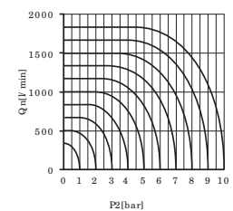
Flow rate orifice spool type
