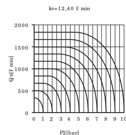
Flow rate orifice spool type
