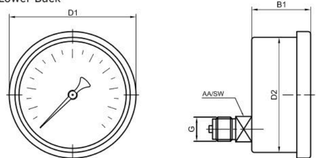
02-Lower Back
