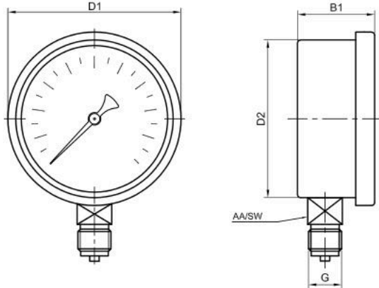
01-Bottom Connection
