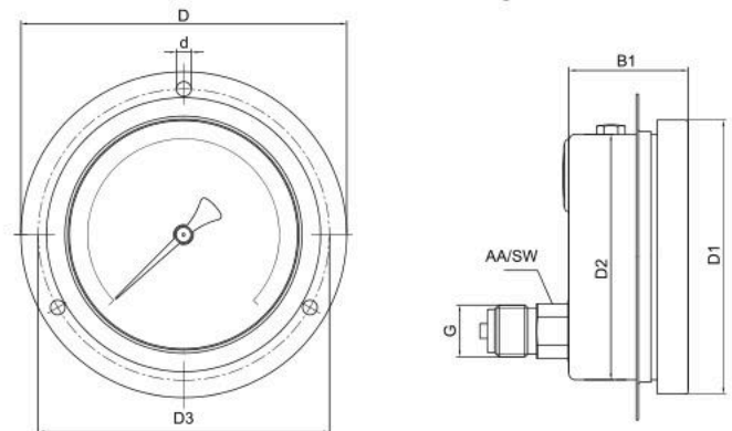
04-03- Lower Back Panel Mount, Front Flange
